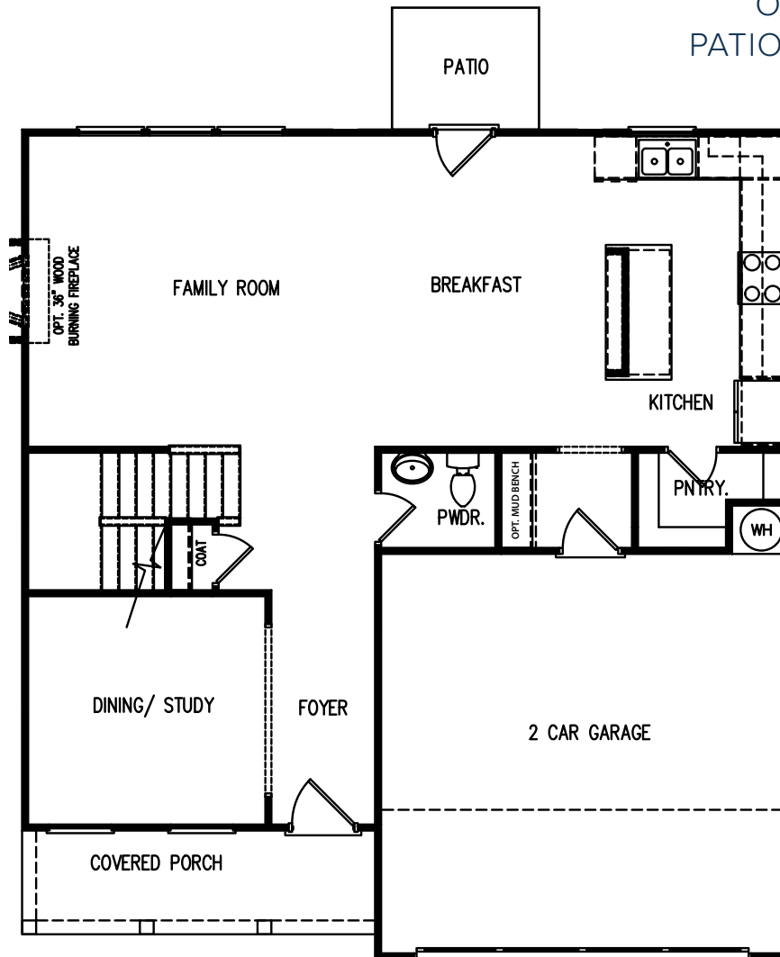
MAIN FLOOR
