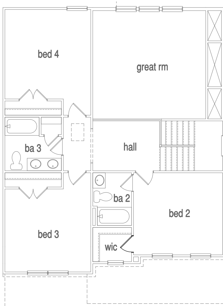
SECOND FLOOR
