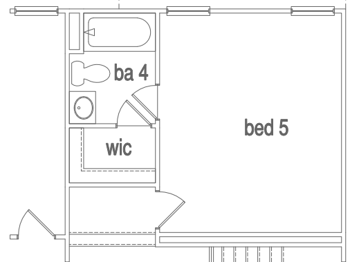
OPT. BED #5 & BATH #4
